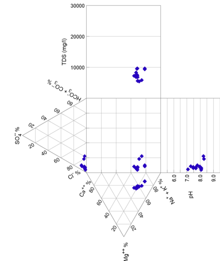
Figure 5.18 Piper and Durov Diagram – Tertiary Sediments
