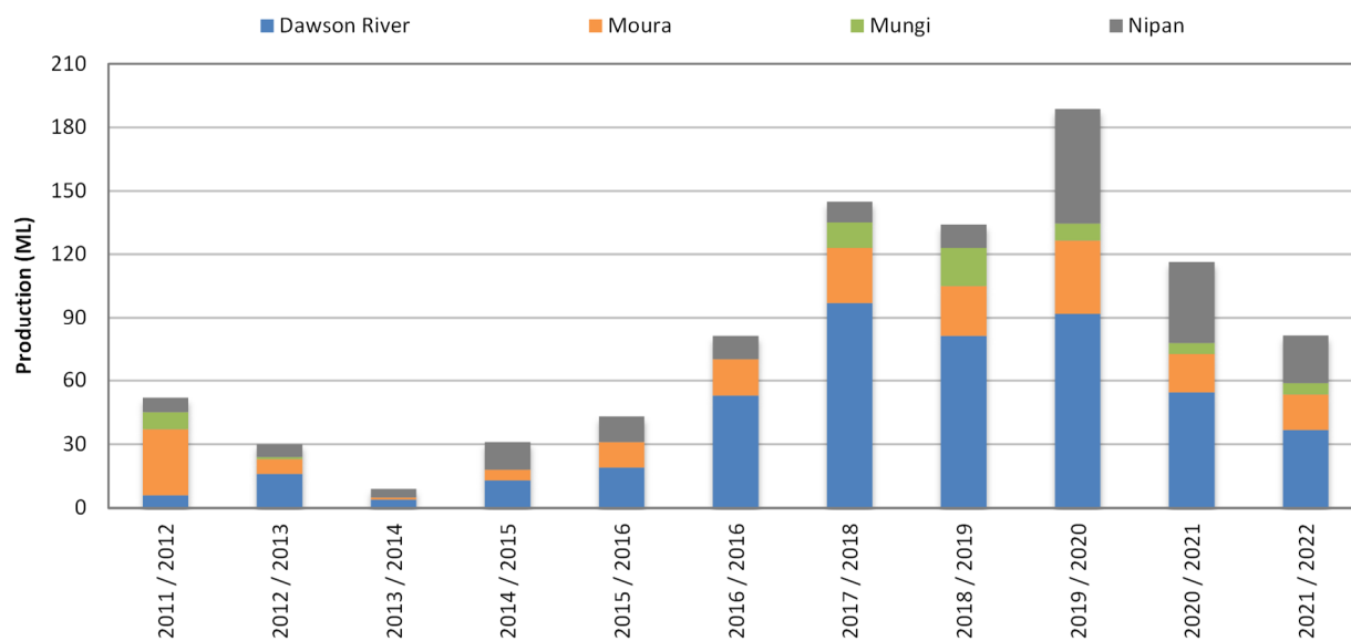
Figure 3.5 PL 94 Historical Water Production
