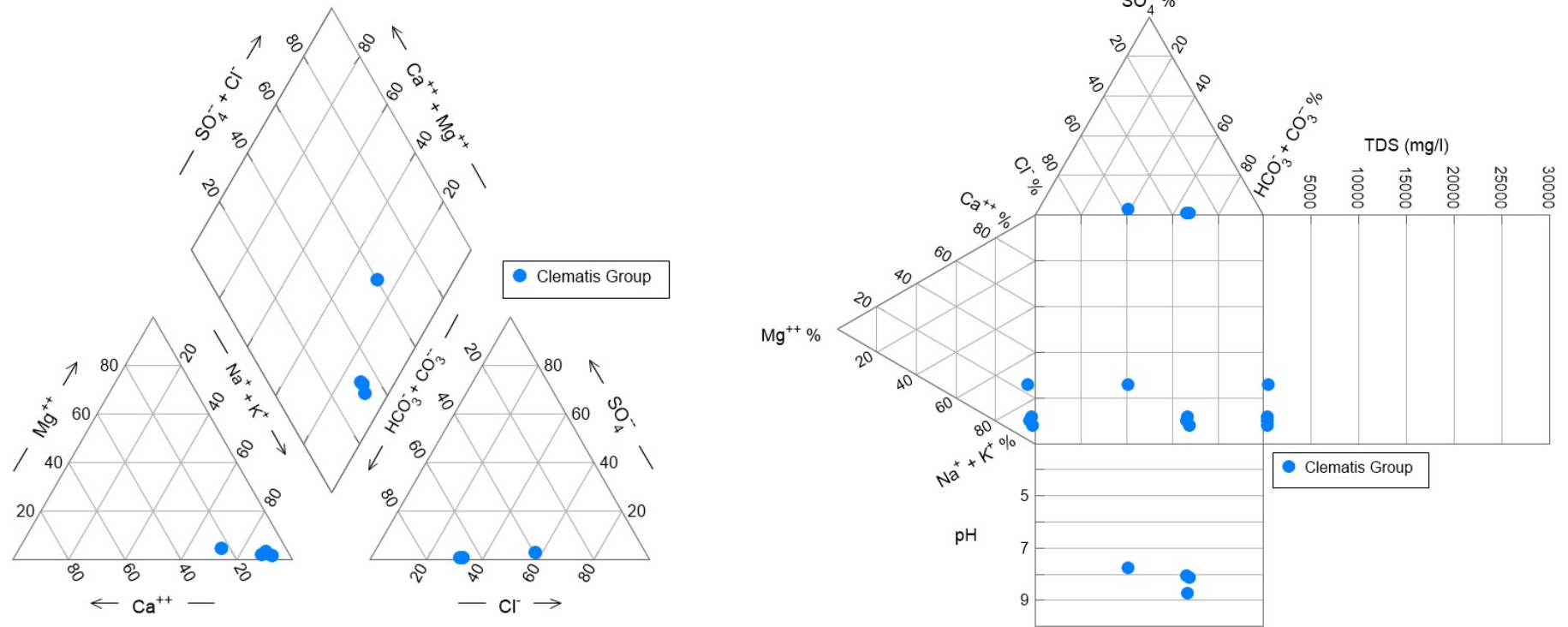
Figure 5.15 Piper and Durov Diagram – Clematis Group
